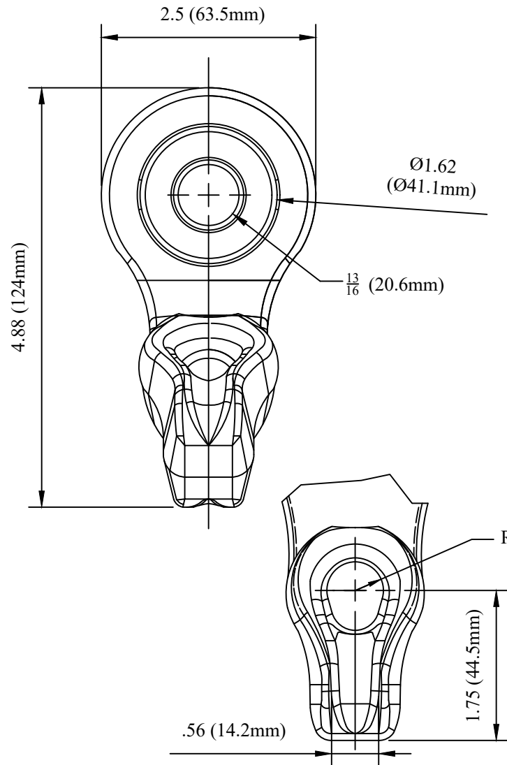
THIMBLEYE DETAIL
